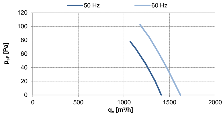
Fan characteristic measured in full bell mouth with guard grill
