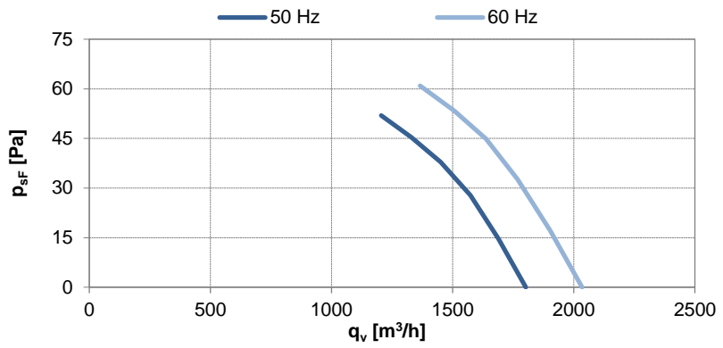
Fan characteristic measured in full bell mouth with guard grill
