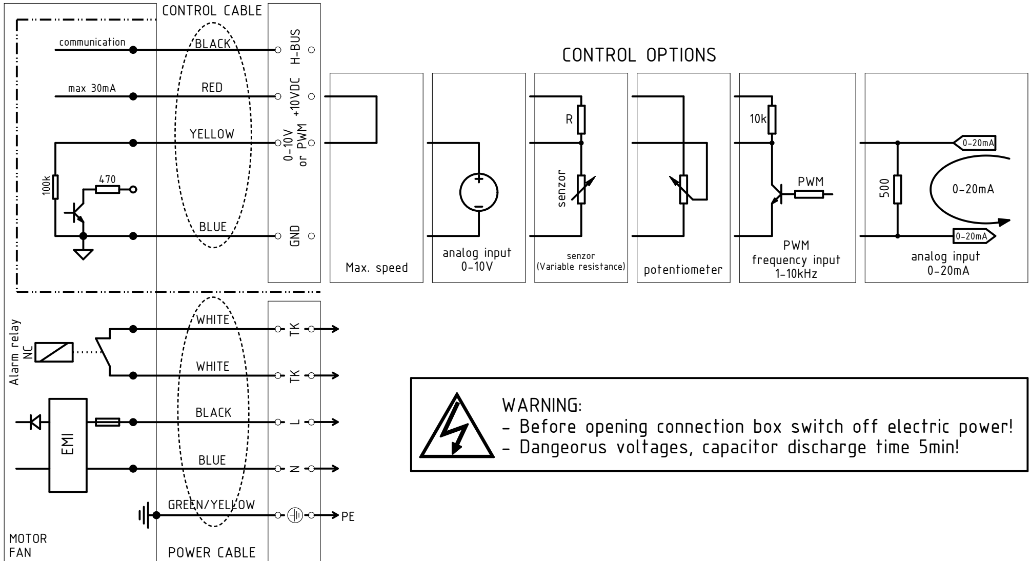
Connecting diagram 0302-0-0001
