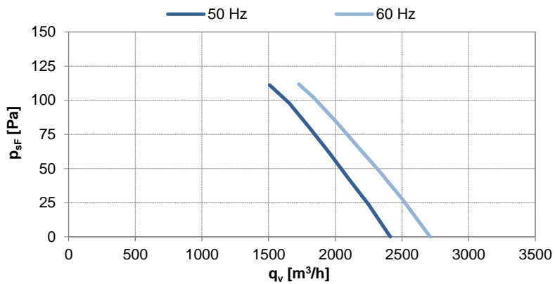
Fan characteristic measured in short bell mouth with guard grill
