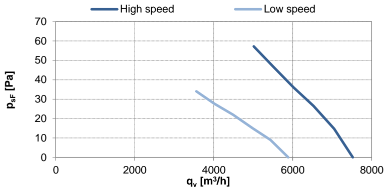
Fan characteristic measured in short bell mouth with guard grill
