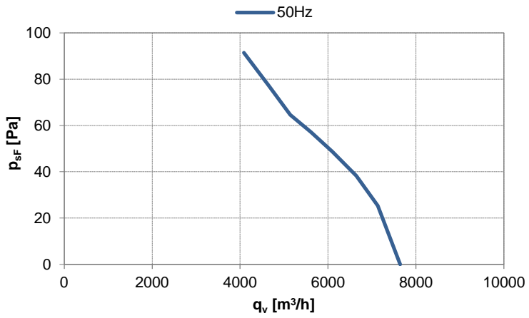
Fan characteristic measured in full bell mouth with guard grill
