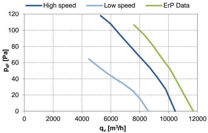
Fan characteristic measured in full bell mouth with guard grill ErP characteristic measured in full bell mouth without guard grill
