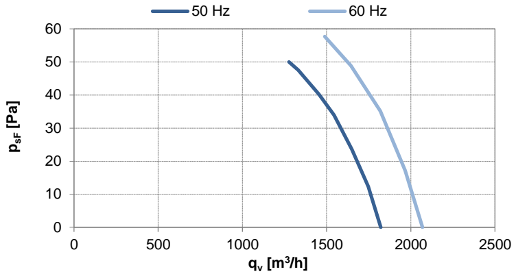
Fan characteristic measured in short bell mouth with guard grill
