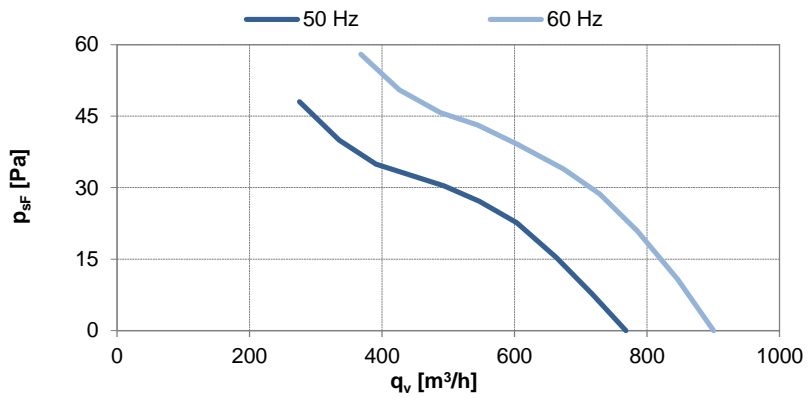
Fan characteristic measured in full bell mouth with guard grill
