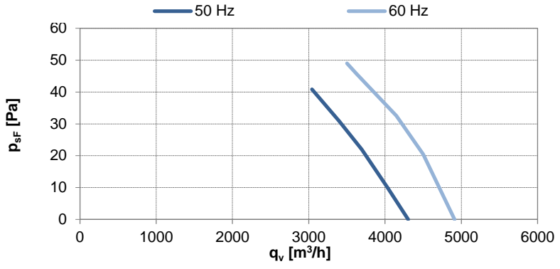
Fan characteristic measured in short bell mouth with guard grill
