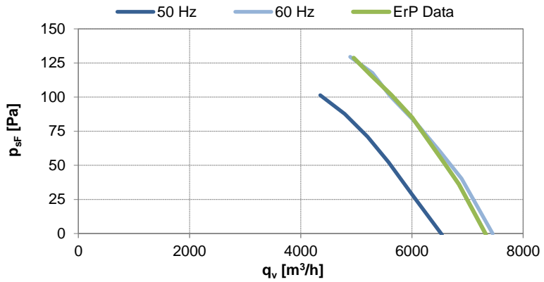
Fan characteristic measured in short bell mouth with guard grill ErP characteristic measured in full bell mouth without guard grill
