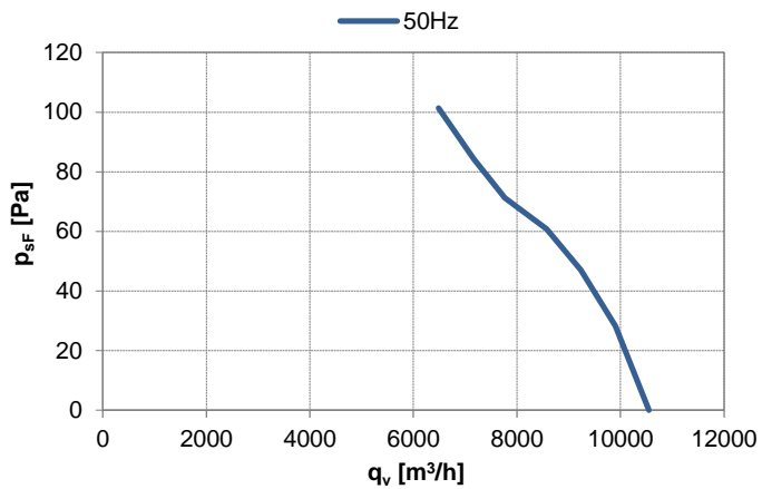
Fan characteristic measured in full bell mouth with guard grill
