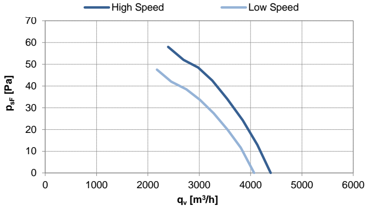
Fan characteristic measured in full bell mouth with guard grill
